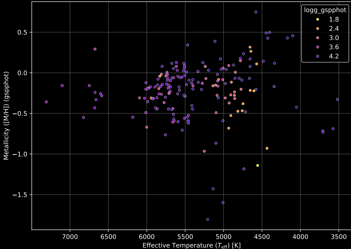
APOGEE DR17 Field: [053+40_MGA] Stellar Population Parameters (n= 180)
