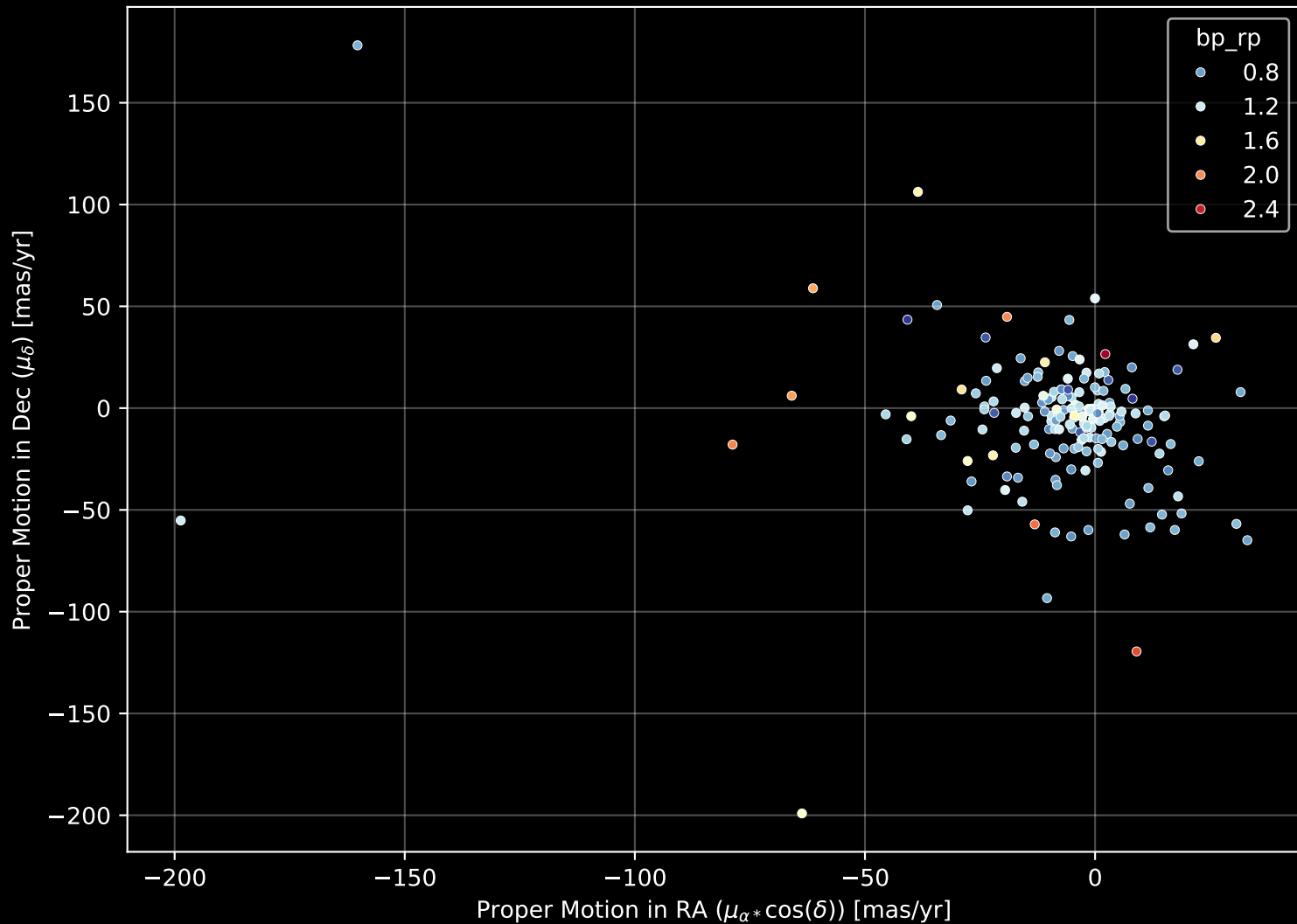
APOGEE DR17 Field: [053+40_MGA] Proper Motion Diagram (n= 180)
