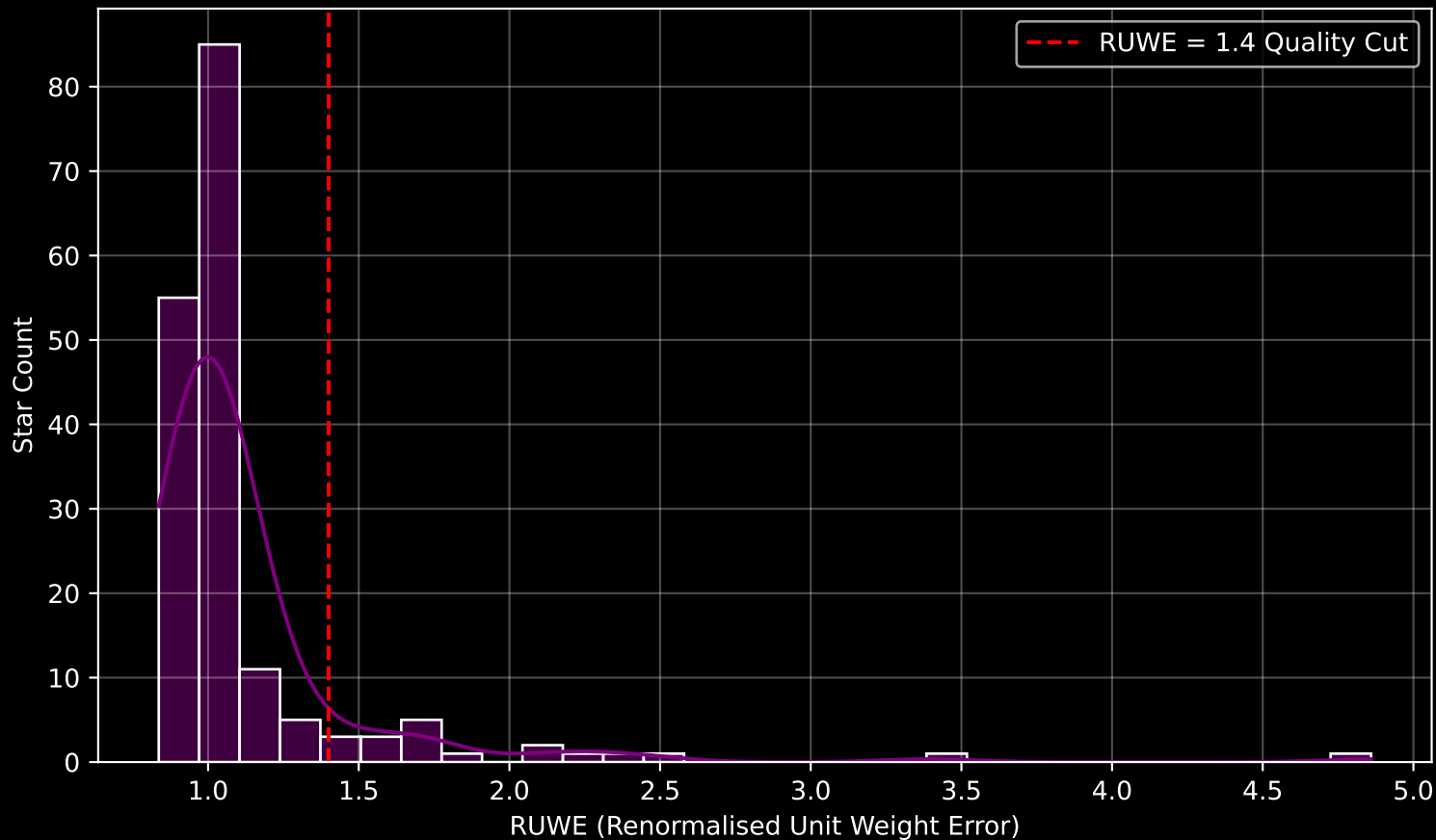
GAPOGEE DR17 Field [053+40_MGA] RUWE Distribution (n= 175)
