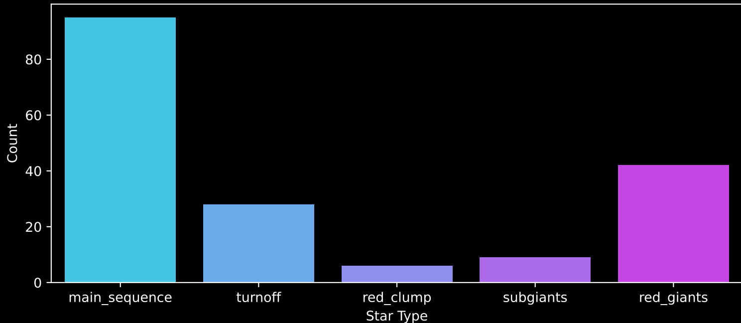
APOGEE DR17 Field: [053+40_MGA] Count plot of Star Type
