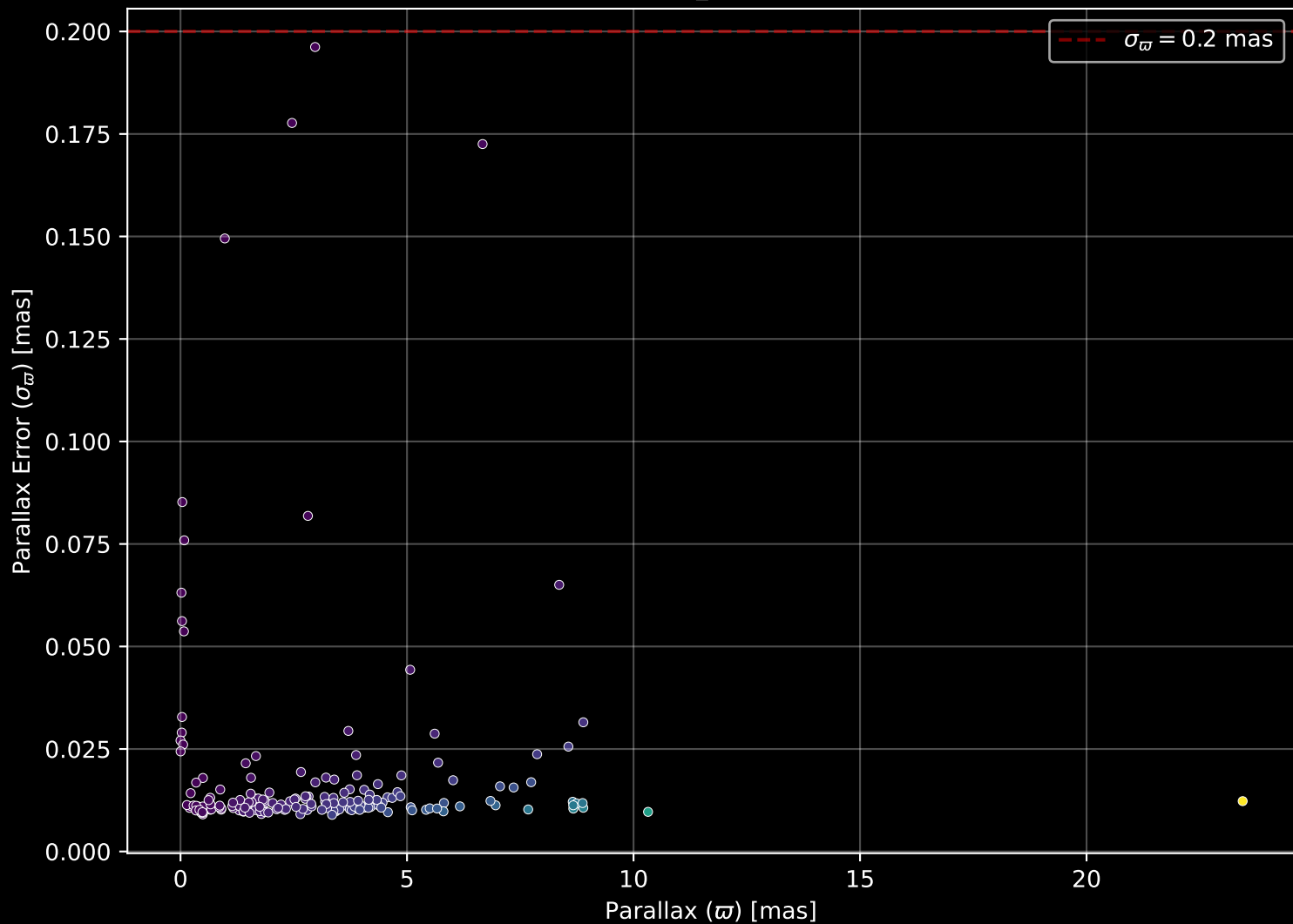
APOGEE DR17 Field: [053+40_MGA] Parallax Quality (n= 180)
